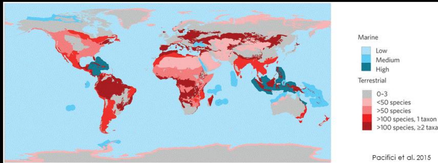
Ecoregional concentrations of climate change vulnerable species
